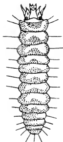
Fig. 421. Lithocolletis hamadryadella Clemens (round form larva).
